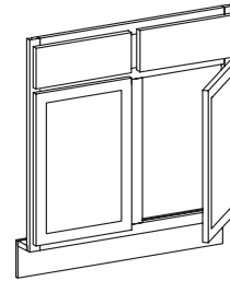
End Stiles 3" Wide, Trimmable 1 1/2" Each End 2 False Drawer Fronts, 2 Doors
