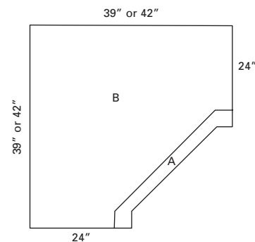
Part A, Front with toekick & part of floor attached. Part B, Floor platform with cleat supports underneath attached. Part A & B mated in field by cabinet installer.
