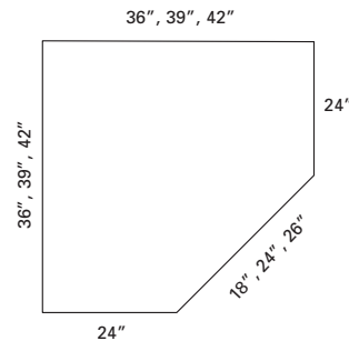
approximate dimensions
